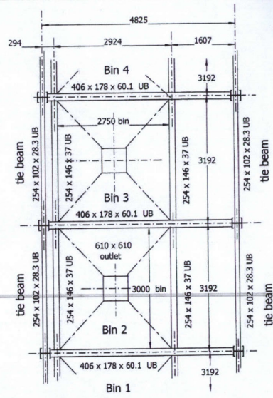
Plan of Steelwork
